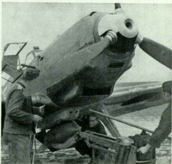
A Luftwaffe Oberfeldwebel supervises the loading of an SC 250 bomb on to a Bf 109E-4/B. Points of interest are the engine crank handle and the armour plate in the side-hinging canopy. This style of spinner decoration was known as "Kullerschнауze".
